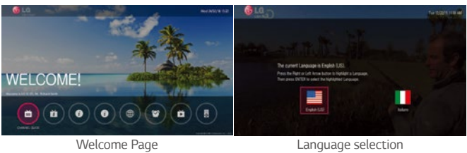
Welcome Page
