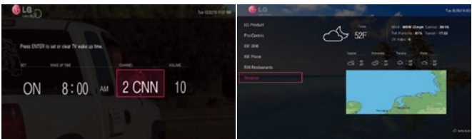
Wake-up Setting
