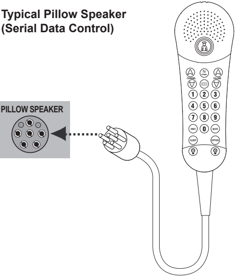
Pillow Speaker Interface Pinout
