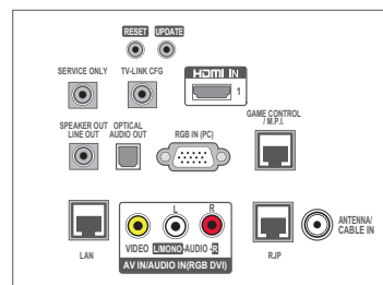
Rear Jack Panel
