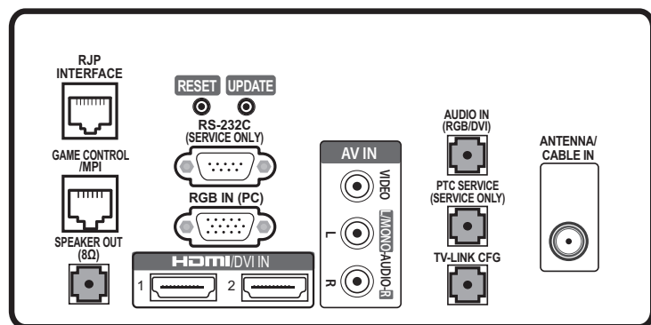
Rear Jack Panel
