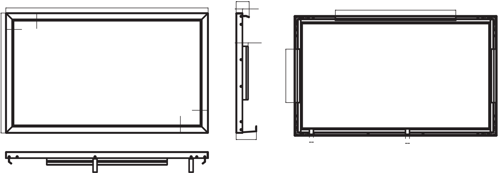
KT-T320 Dimension
