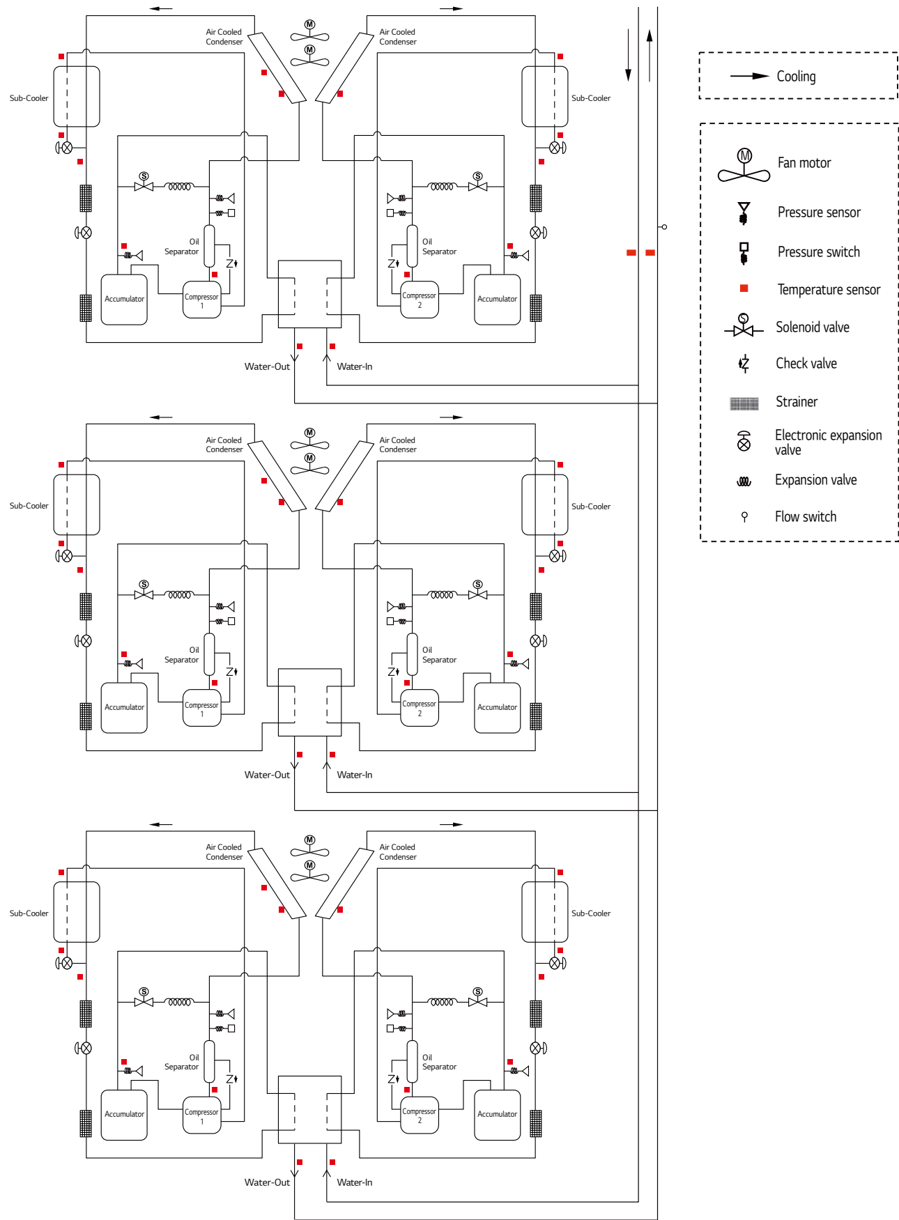
ACAH Series 3 Unit
