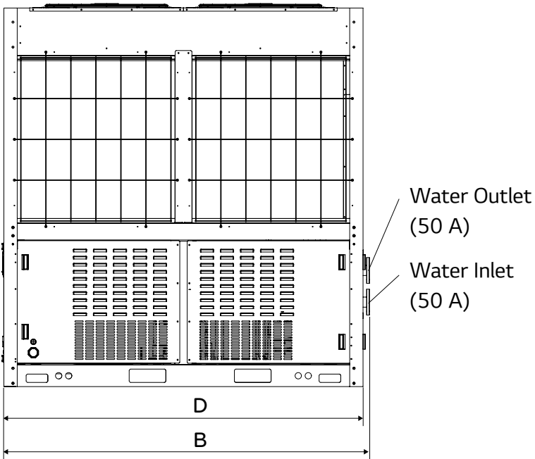
Side view
