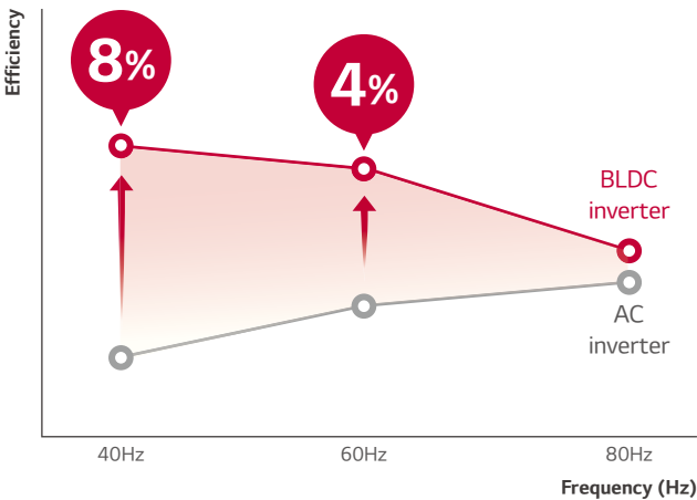
Motor Efficiency
