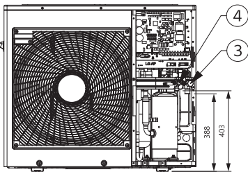
Piping Connection Port
