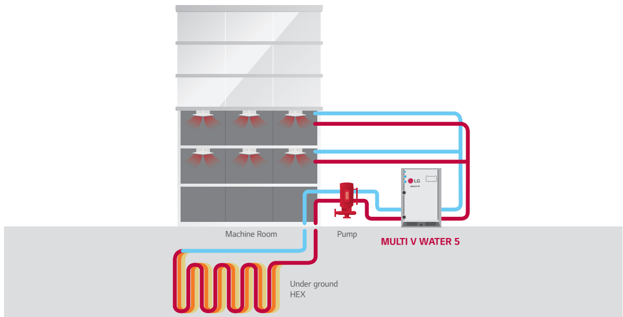
Chiller - FCU
