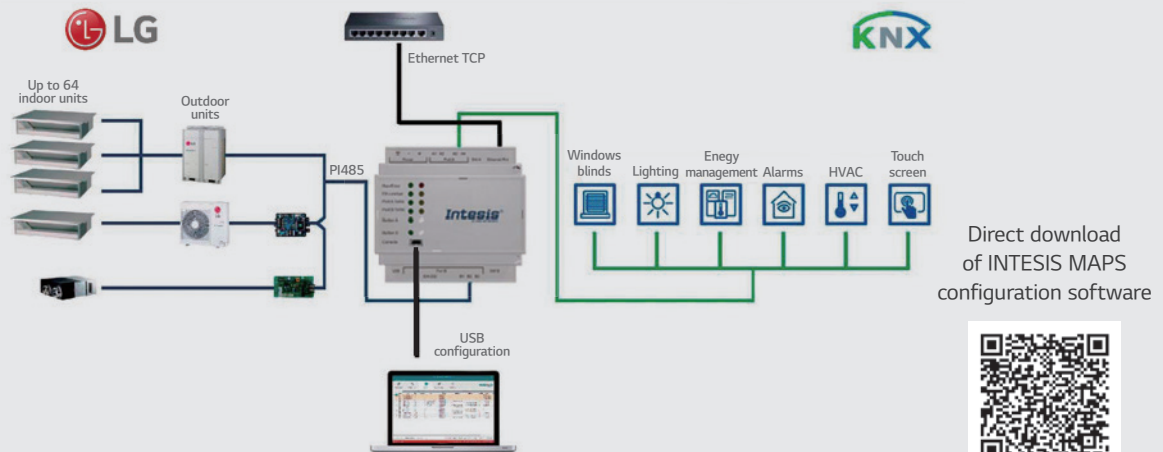
Integration of LG VRF systems into KNX control systems
